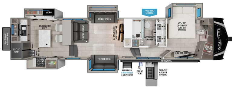
390RK U W 1 14,562 HITCH 1 2,794 GVWR 18,000 LENGTH 2 42' 5" HEIGHT 3 13' 5" CAPACITY 81 106 53
