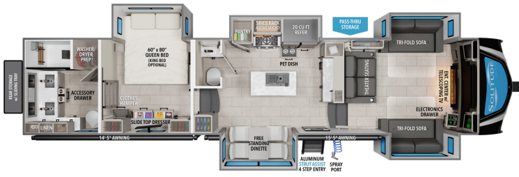
380FL U W 1 14,866 HITCH 1 3,052 GVWR 18,000 LENGTH 2 41' 4" HEIGHT 3 13' 5" CAPACITY 81 106 106
