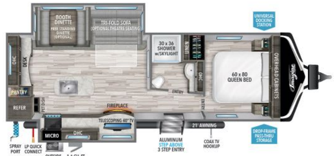
2670MK UVW' 6,845 HITCH' 690 LENGTH' 32' 3" HEIGHT 11' 1" CAPACITY 52 82 45
