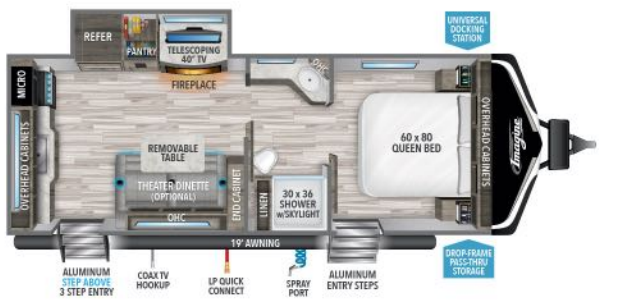
2250RK UVW' 5,546 HITCH' 515 LENGTH' 27' 11" HEIGHT 11' 0" CAPACITY 52 90 45
