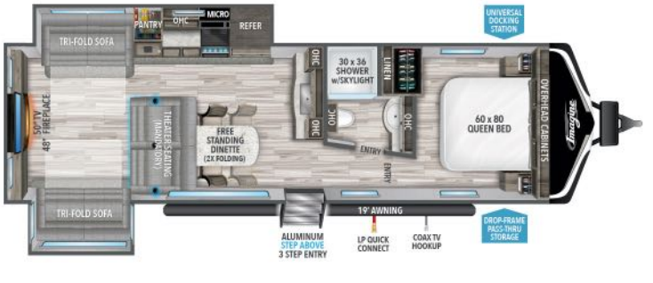
3100RD UVW' 7,778 HITCH' 791 LENGTH' 35' 11" HEIGHT 11' 2" CAPACITY 52 90 45
