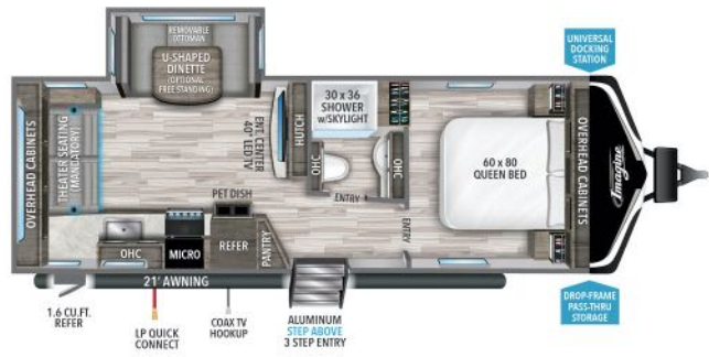
2450RL UVW' 5,834 HITCH' 580 LENGTH' 29' 11" HEIGHT 11' 0" CAPACITY 52 90 45
