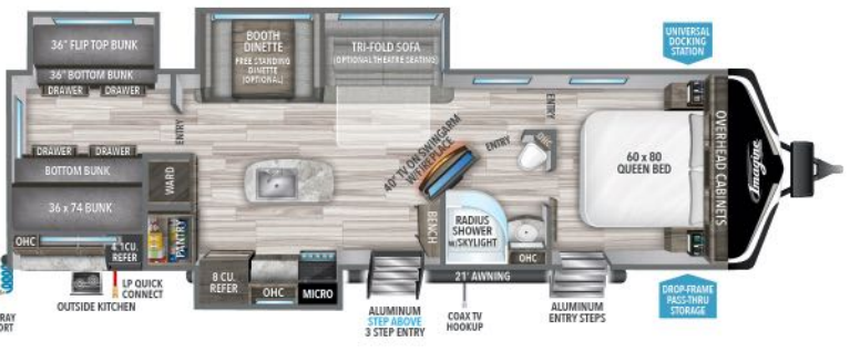
3250BH UVW' 8,496 HITCH' 844 LENGTH' 36' 11" HEIGHT 11' 4" CAPACITY 52 90 45
