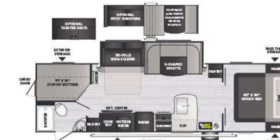
2951BH | Multi-purpose bunkhouse w/ outside kitchen
