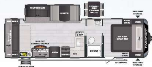
2700RL | Rear living, 60 x 80 queen bed
