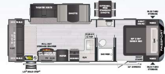
2700RLWE | Rear living, 60 x 80 queen bed
