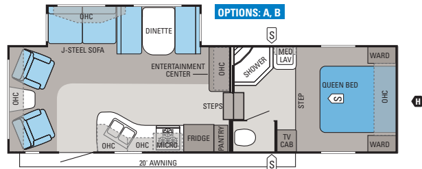
SUPER LITE FIFTH WHEEL | 28.5RLS
