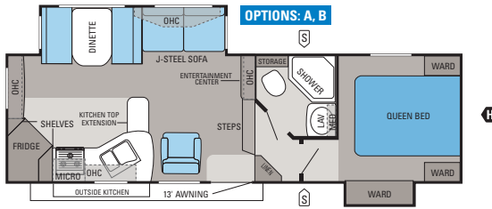
SUPER LITE HALF-TON FIFTH WHEEL | 26.5RKS
