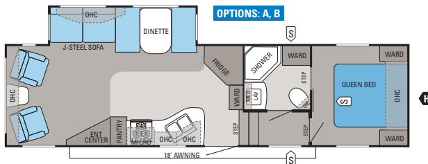
SUPER LITE FIFTH WHEEL | 30.5RLS
