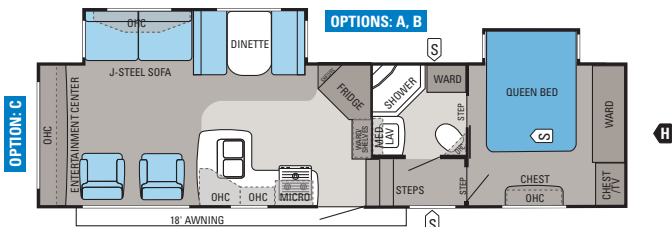
SUPER LITE FIFTH WHEEL | 31.5RLDS
