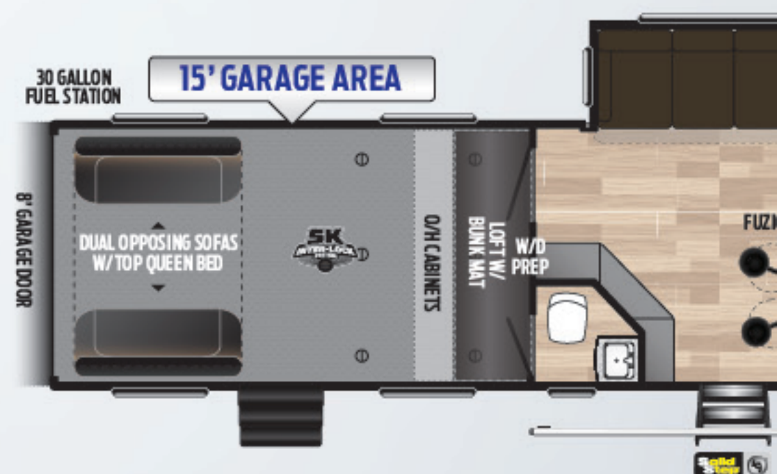
NEW! 415 | TRIPLE-AXLE, 15' GARAGE, 12 CU. FT. REFER
