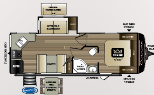
24SABWE | Dual Entry Rear Kitchen with Slide Weight: 6061 LBS. | Length: 28' 4"
