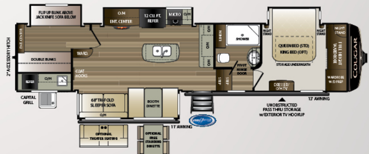
369BHS | Bunkhouse, large outside kitchen Weight: 11547 LBS. | Length: 39' 4"
