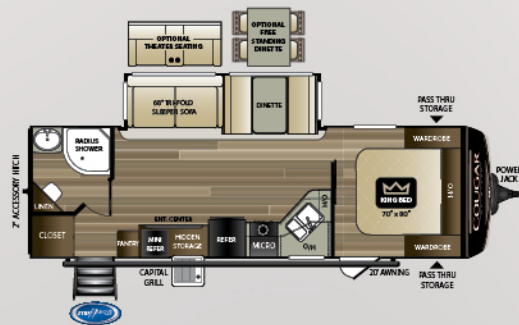
26RBSWE | Rear Bath with Slide and Outside Kitchen Weight: 6471 LBS. | Length: 30' 5"
