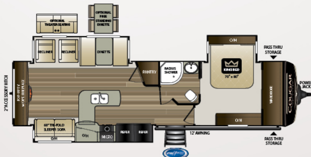
33SAB | Rear entertainment, double refrigerator Weight: 8847 LBS. | Length: 36' 11"
