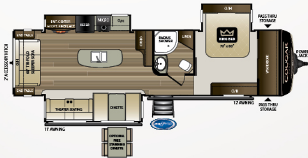
32RLI | Rear living room, three slides w/ bedroom slide Weight: 8416 LBS. | Length: 35' 11"
