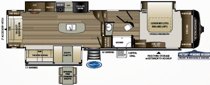
361RLW | Master suite, rear-living w/ windshield Weight: 11269 LBS. | Length: 39' 4"
