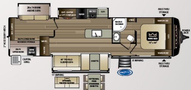
34TSB | Three-slide bunk house w/ outside kitchen Weight: 8563 LBS. | Length: 37' 5"
