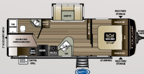
25BHSWE | Short Double Bunk House with Outside Kitchen Weight: 6073 LBS. | Length: 29' 4"
