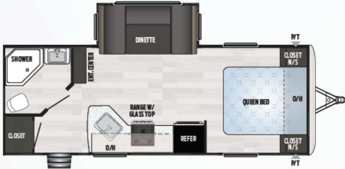
212RBWE | Small slide, rear bath Weight: 5270 LBS. | Length: 25' 11"
