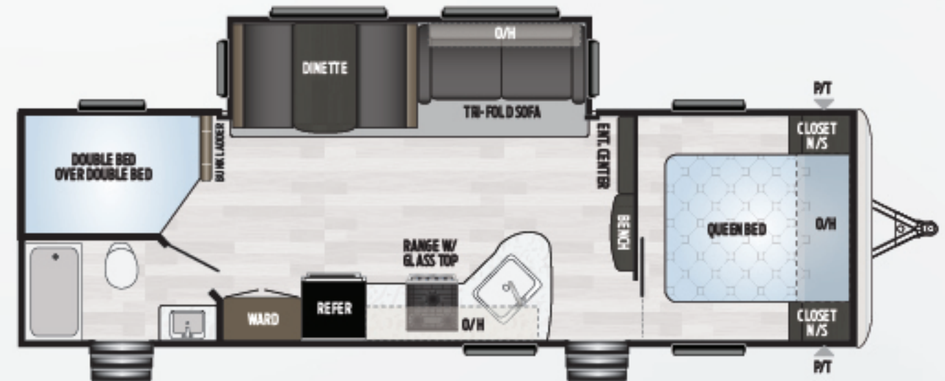
282BHWE | Large slide, double bunks, private bedroom Weight: 6960 LBS. | Length: 32' 1"
