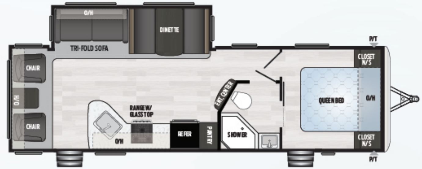
271RLWE | Large slide, rear living, chairs, dual entrance Weight: 6731 LBS. | Length: 31' 10"
