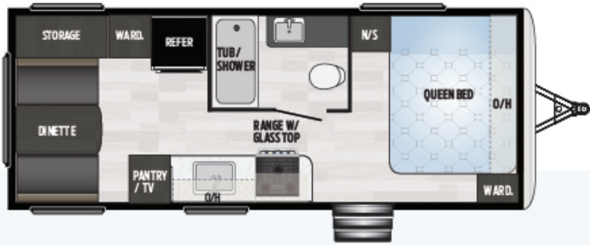
179QBWE | Non slide, queen bed Weight: 3983 LBS. | Length: 21' 10"
