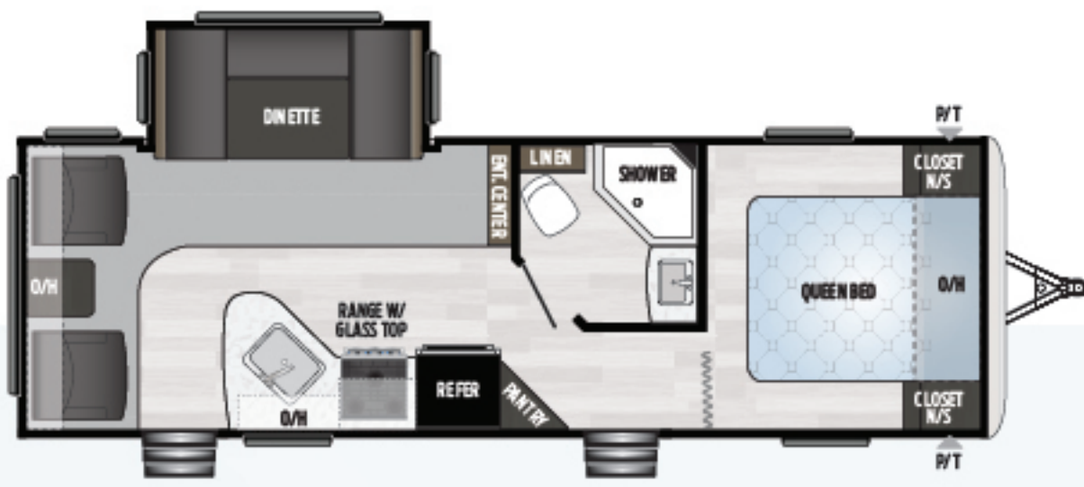
258RLWE | Small slide, rear living, chairs Weight: 6007 LBS. | Length: 29' 7"
