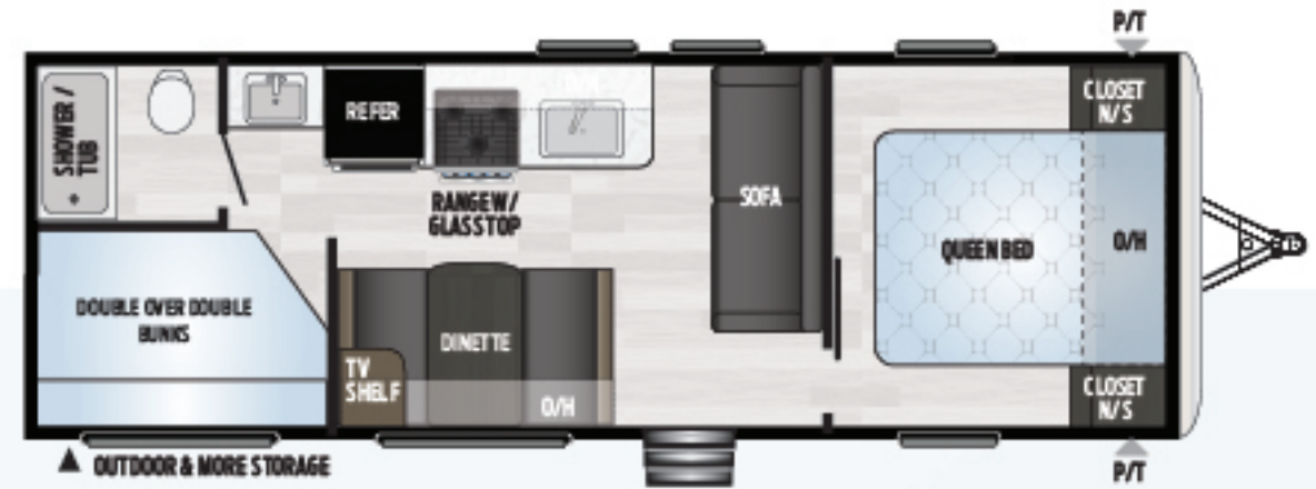
260TBWE | Non slide, double bunks, private bedroom Weight: 4883 LBS. | Length: 28' 6"
