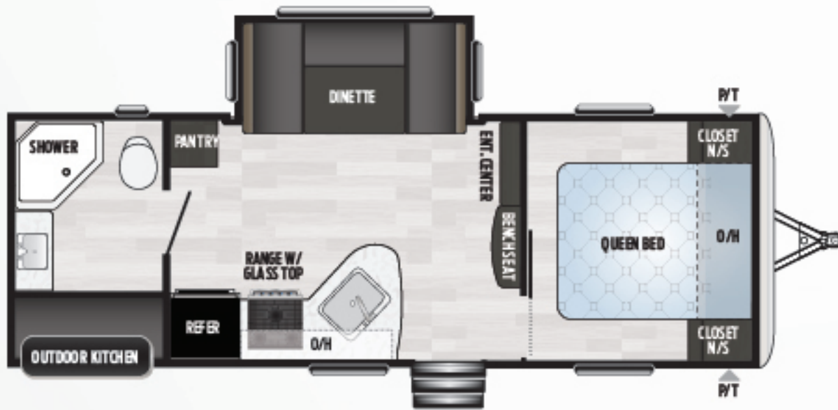
235RBWE | Small slide, rear bath, outdoor kitchen Weight: 5851 LBS. | Length: 27' 5"
