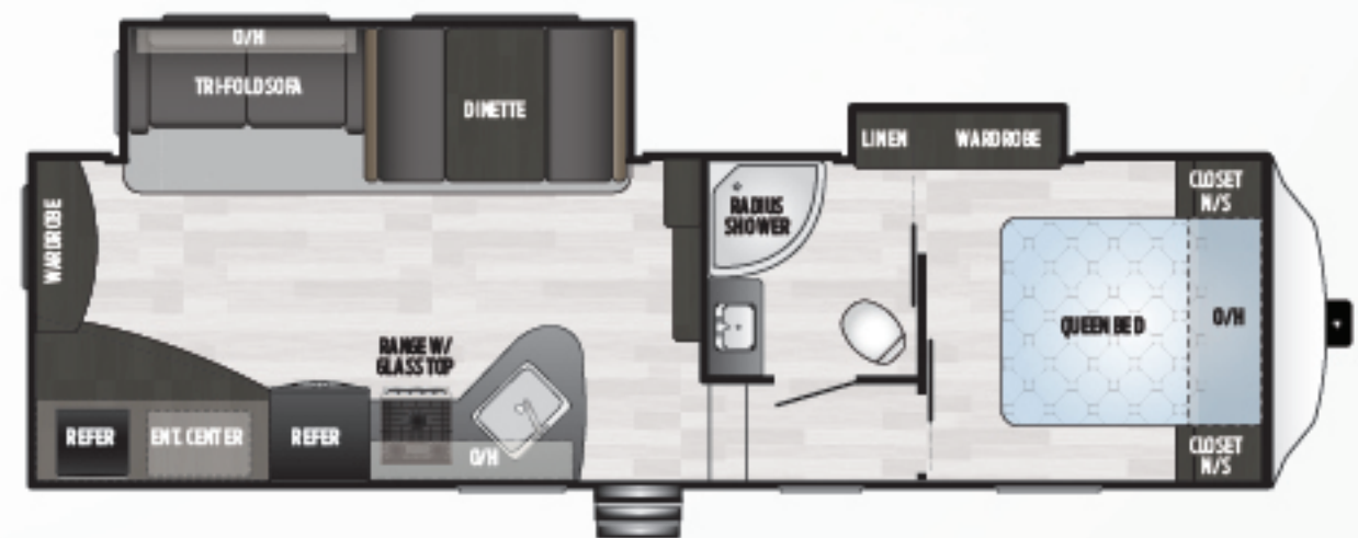
272FWRE | 2 slides, rear entertainment, outside kitchen Weight: 7775 LBS. | Length: 30'2"
