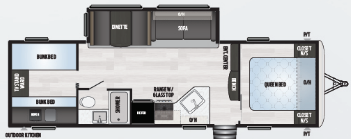
298BHWE | NEW Private bunkroom, private master bedroom, outside kitchen Weight: 6860 LBS. | Length: 32' 8"
