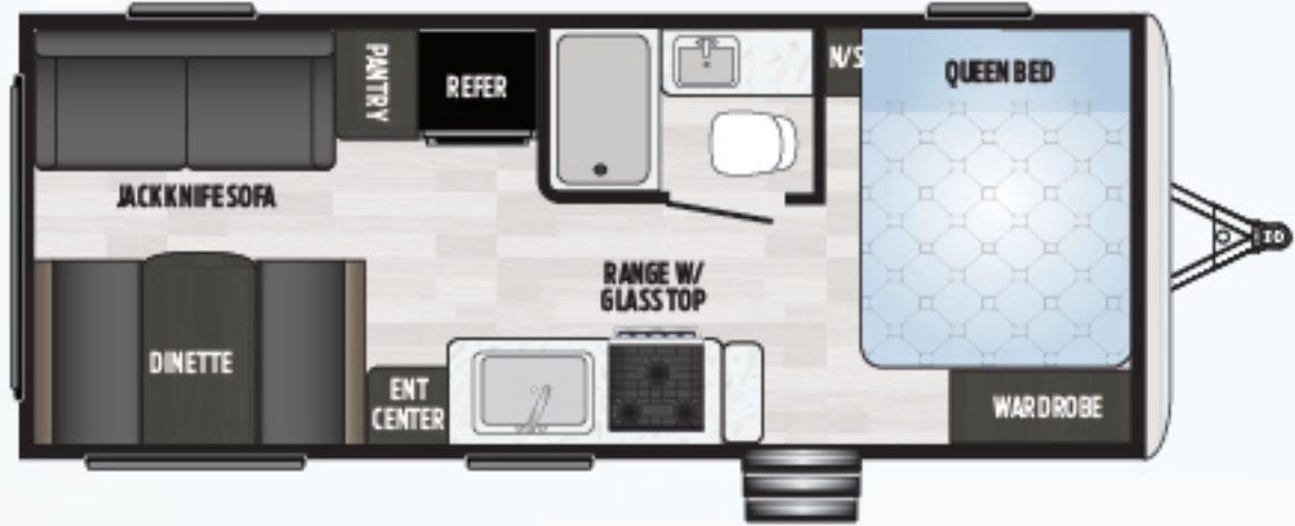
201RDWE | Non slide, rear dining Weight: 4307 LBS. | Length: 24' 0"
