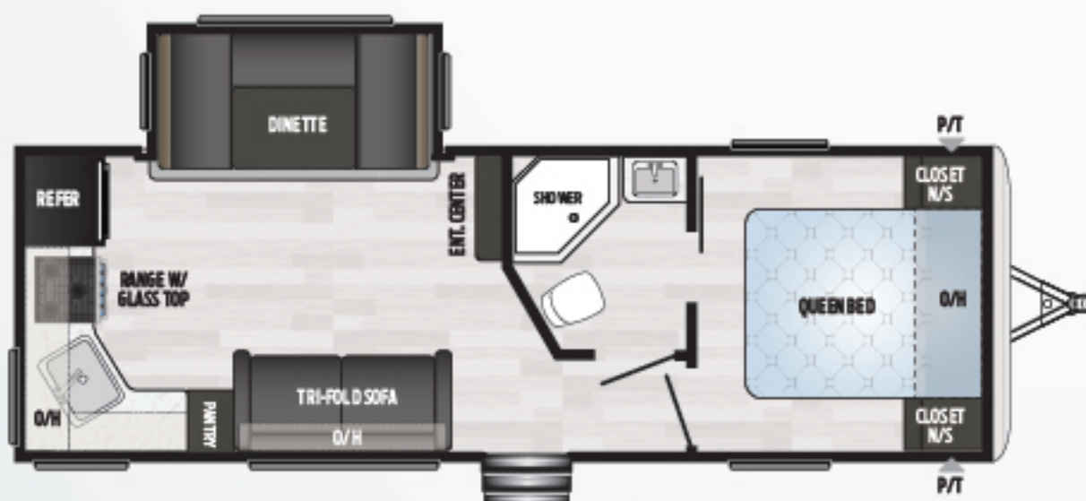
242RKWE | Small slide, rear kitchen, dual entry bath Weight: 5784 LBS. | Length: 28' 6"
