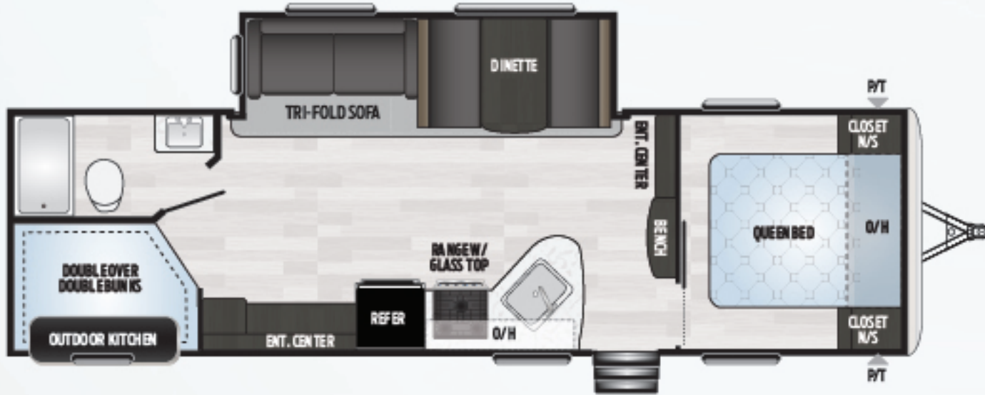
270BHWE | Large slide, double bunks, outdoor kitchen Weight: 6903 LBS. | Length: 32' 11"
