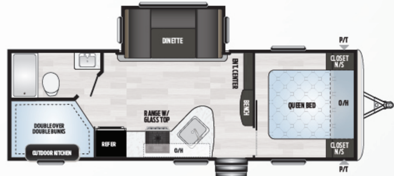
240BHW | Small slide, private bedroom, double bunks Weight: 5765 LBS. | Length: 28' 11"
