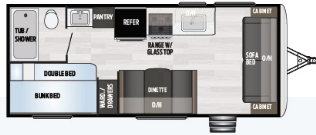
189FLWE | Non slide, front living Weight: 4242 LBS. | Length: 23' 7"
