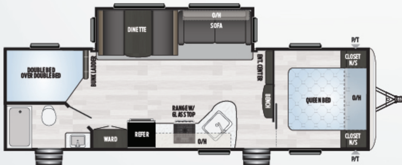
282BHSEWE | Large slide, double bunks, private bedroom STOCK ONLY Weight: 6550 LBS. | Length: 32' 1"
